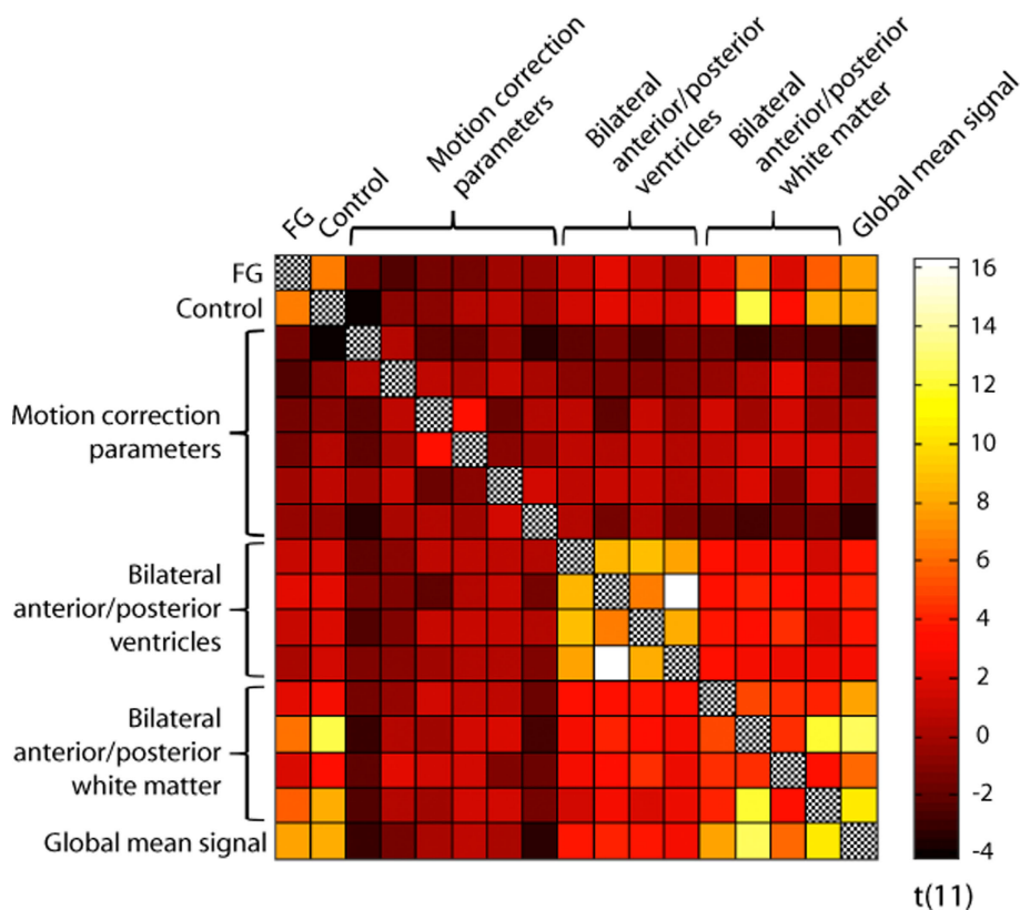
FIGURE A2 | Group confusion matrix from Experiment 1. Crosscorrelation of all regressors from resting run models for each subject (concatenating regressors across runs within subject), converted to z-scores using Fisher's r -to- z transformation, and evaluated across subjects with one-sample t -tests.
