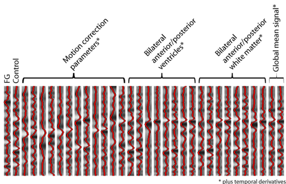
FIGURE A1 | Example resting run model from Experiment 1. Resting timeseries were extracted from the localized FG and control seed regions, and entered into a multiple regression model of the same resting run with several nuisance regressors of no interest.
