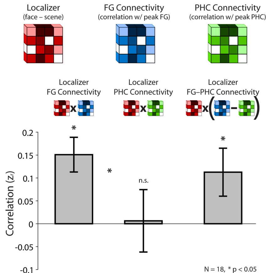
FIGURE 5 | Pattern analysis from Experiment 2. Across a population of pSTS voxels, correlations between the strength of face-selectivity from the localizer and the strength of resting connectivity with the peak FG (after partialing out the PHC) and the peak PHC (after partialing out the FG). Voxels that were more face-selective in the localizer were also more correlated with the FG at rest, but
